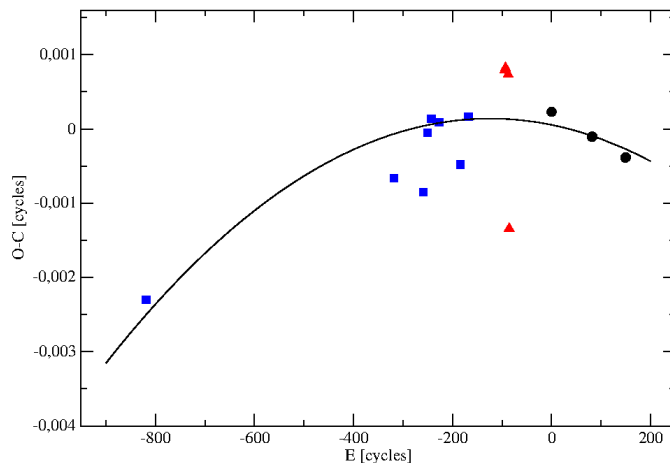
Fig. 9. The O - C diagram for the moments of eclipses in V2080 Cyg based on data collected between 1998 and 2011. Black circles represent our dataset, data taken from the SuperWASP are shown with red triangles, and blue squares correspond to data provided by İbanoğlu et al. (2008).
