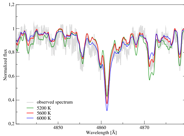
Figure 10: The comparison of the combined spectrum (gray color) and synthetic (with different colors) of the H_{\beta} region. Different colors correspond to synthetic spectra calculated for various effective temperatures within the limits of error.
