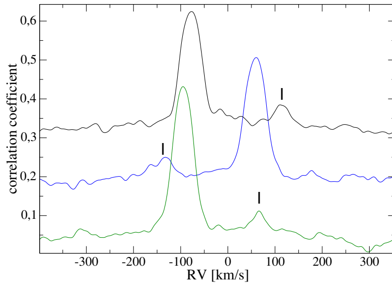
Fig. 2. Cross-correlation function of BD-00 2862 for different phases. The small peak of the secondary component is marked.
