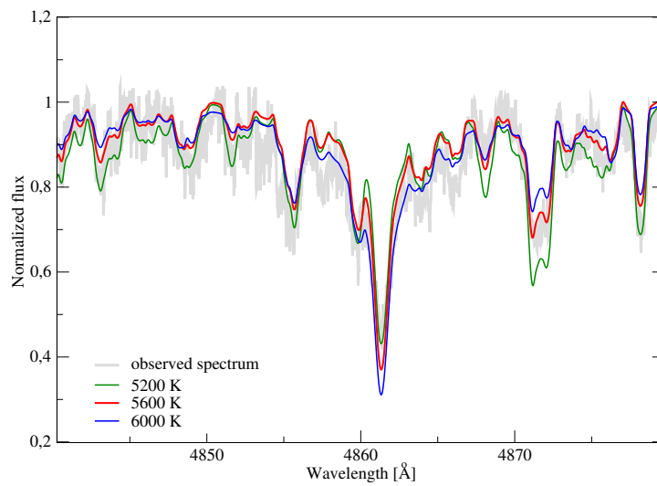
Figure 10: The comparison of the combined spectrum (gray color) and synthetic spectrum (with different colors) of the H_\beta region. Different colors correspond to synthetic spectra calculated for various effective temperatures within the limits of error.
